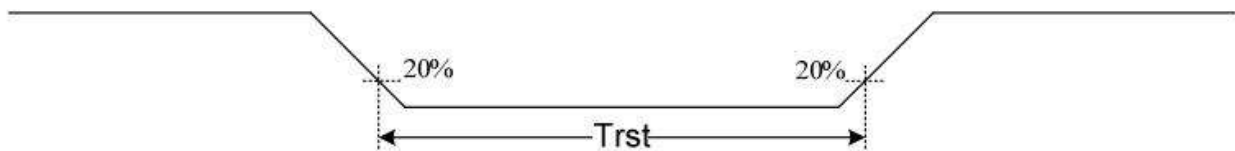
Figure 13.5: Reset timing
