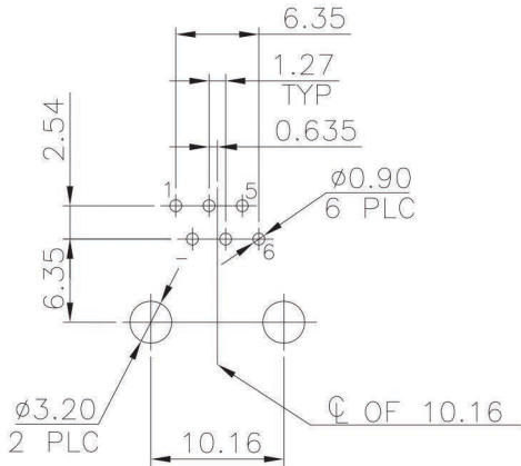
Recommended PCB Layout (Component Side)
