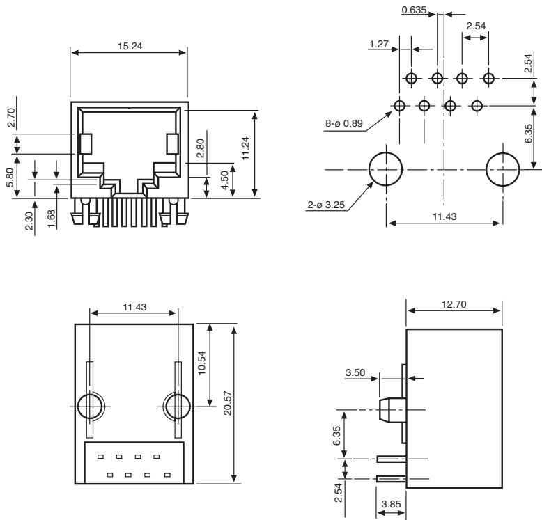
PCB Hole Pattern
