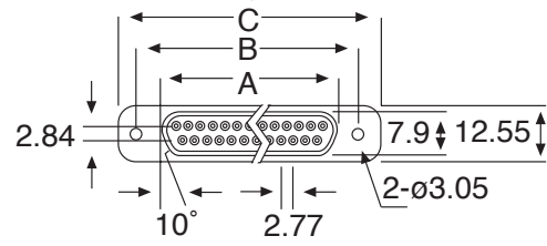
SOCKET (9 - 37 way)
