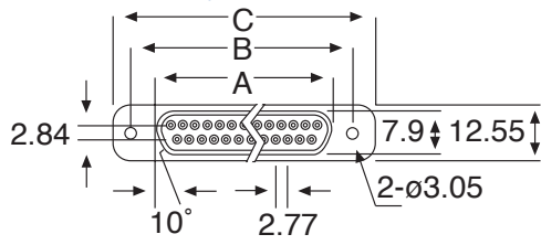
PLUG (9 - 37 way)
