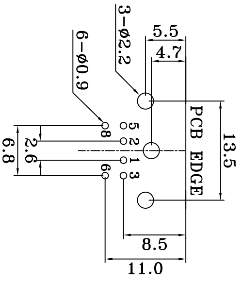
PCB LAYOUT (BOTTOM VIEW)
