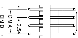
(2 through 5 circuits)
