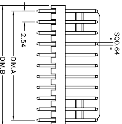
(6 through 20 circuits)
